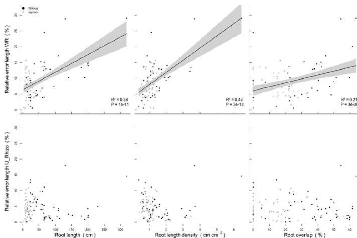
Figure 3: Relationships between the magnitude of the relative error in root length and the root length, root length density and root overlap for WinRhizo TM and IJ_Rhizo at 1200 dpi with fixed threshold. Errors are absolute of (Estimate-Correct)/Correct*100. All three explanatory variables correlated positively with each other in our dataset.
